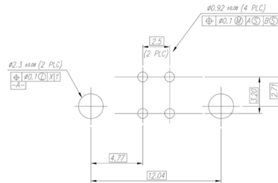
FIGURE A: PCB FOOTPRINT FOR RECEPTACLE (THROUGH-HOLE)
