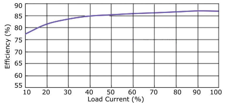
AE40-EW-S24 Efficiency Curve Efficiency vs. Load Current
