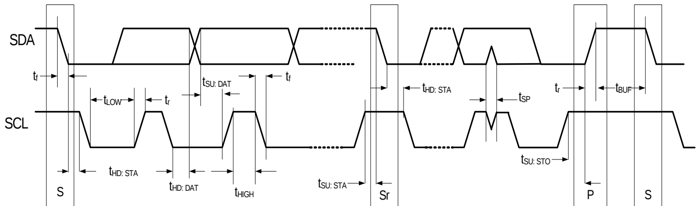
Figure 13. Definition of I2C Bus Timing
