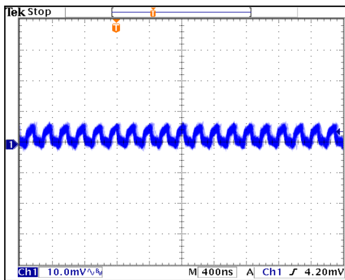
Ripple Voltage, 3.3V_{IN}/1.2V_{OUT} , I_{OUT}=9A , C_{OUT} = 5 \times 22\mu F
