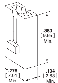
Cavity Specification 1601425
