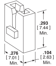
Cavity Specification 1601434
