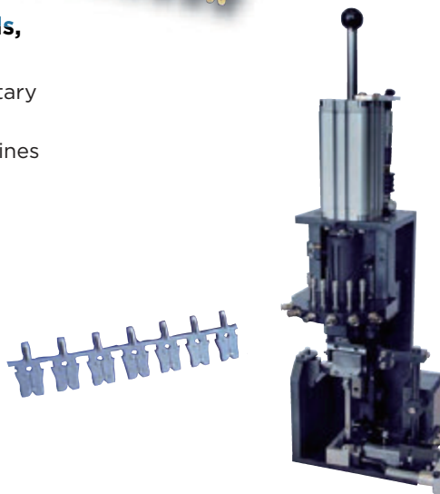
Pneumatic Insertion Tool
