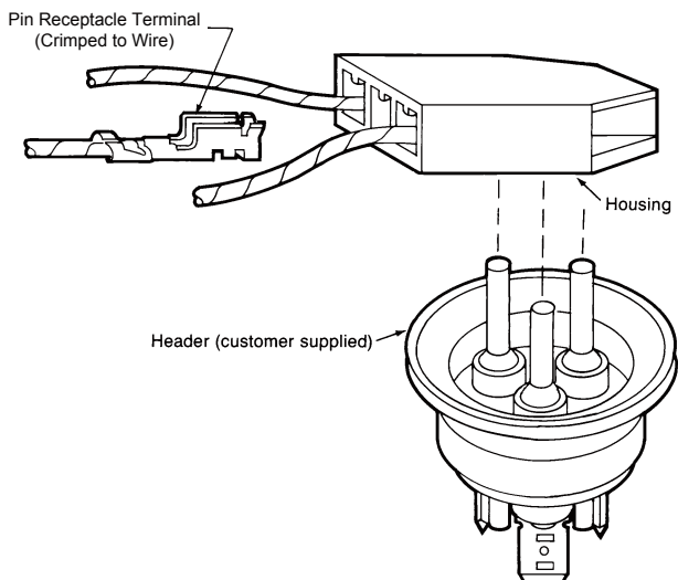
Typical Assembly
