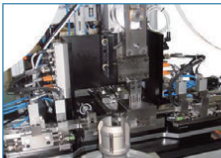
Horizontal Design
