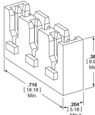
Cavity Specification 1601440
