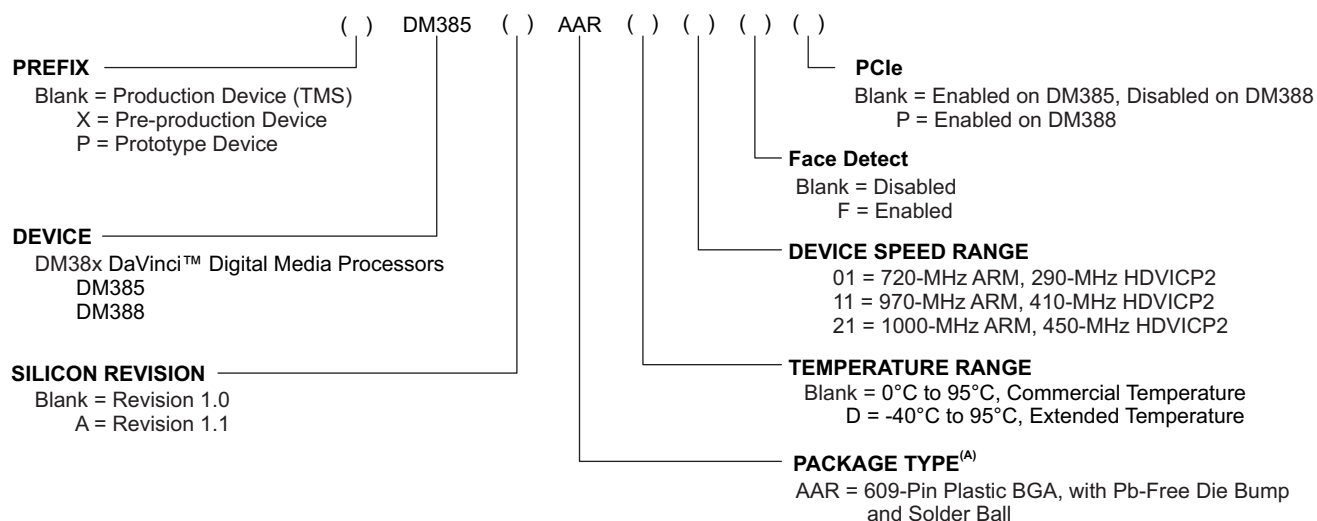
Figure 9-1. Device Nomenclature
