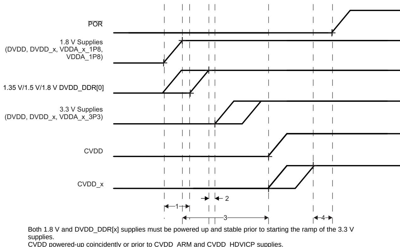
Figure 7-1. Power-Up Sequence
