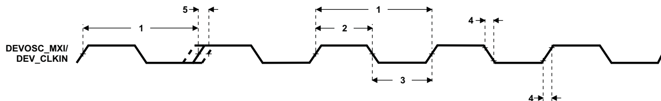
Figure 7-13. DEV_MXI/DEV_CLKIN Timing
