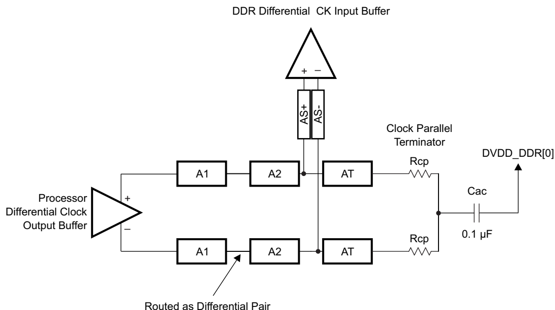
Figure 8-72. CK Topology for One DDR3 Device
