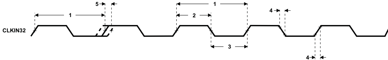
Figure 7-15. CLKIN32 Timing
