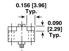
TYPICAL END VIEW 34 THRU 50 CONTACTS
