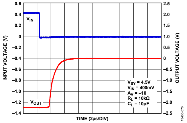
Figure 70. Negative Overload Recovery, V_{SY} = 4.5\text{ V}
