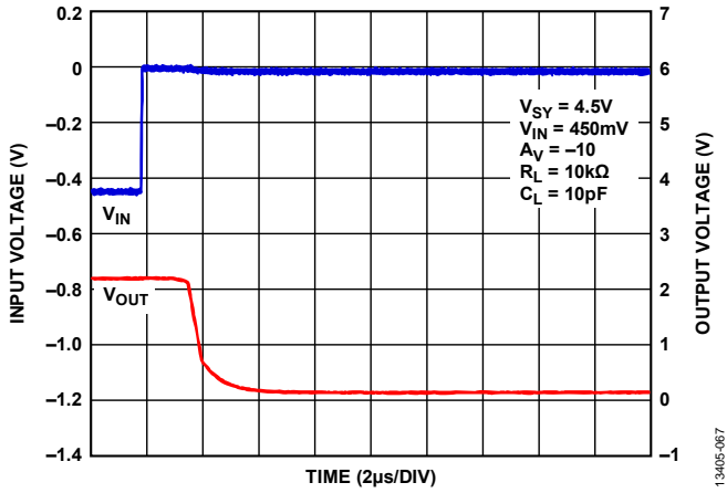
Figure 67. Positive Overload Recovery, V_{SY} = 4.5\text{ V}
