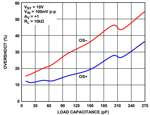
Figure 60. Small Signal Overshoot vs. Load Capacitance
