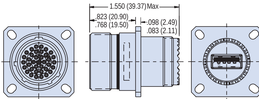
Square Flange Receptacle
