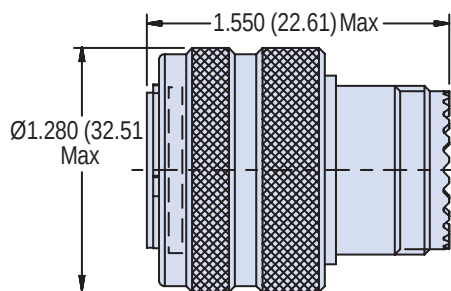
Plug
