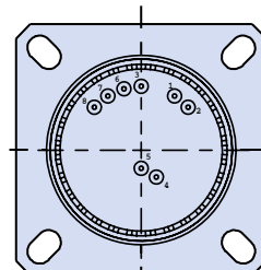
Receptacle Rear View Size #22 Crimp
