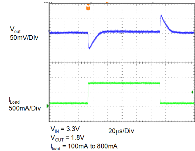
Transient Response
