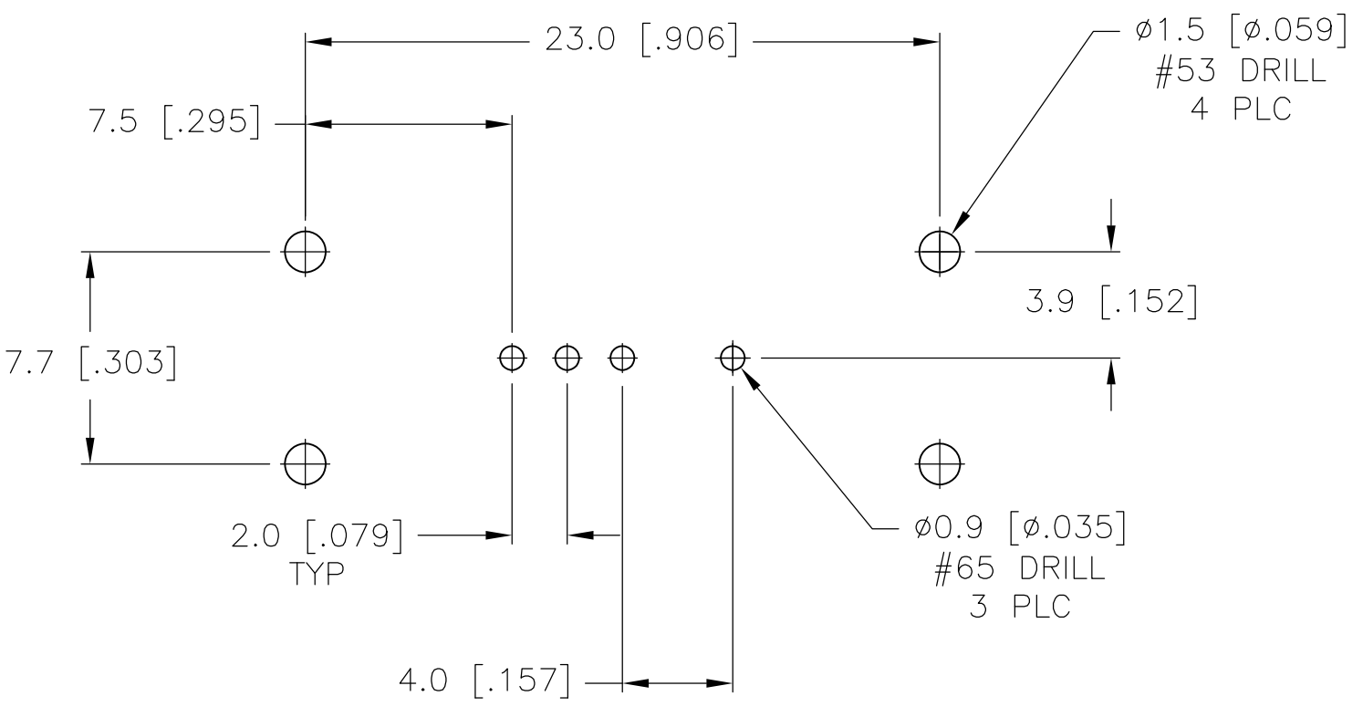
RECOMMENDED BOARD LAYOUT
