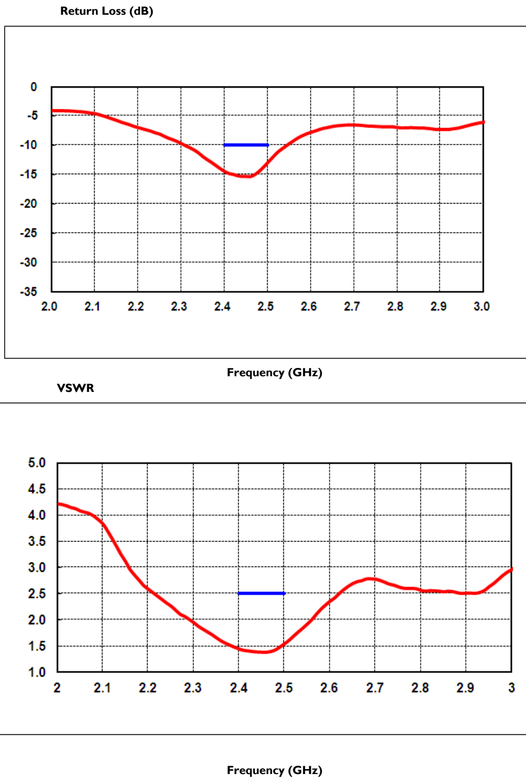
Fig. 2 Return loss & VSWR Measurement
