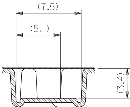
SECT:X-X (SCALE 4:1)
