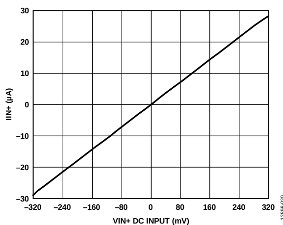
Figure 20. I_{IN+} vs. VIN+ DC Input
