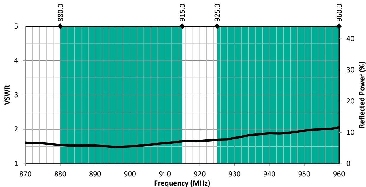
Figure 1. CW LTE Band 8 Antenna VSWR with Band 8 Uplink/Downlink Highlights
