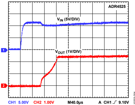
Figure 18. ADR4525 Output Voltage Start-Up Response
