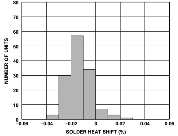
Figure 42. ADR4530 Solder Heat Resistance Shift (3 × Reflow)
