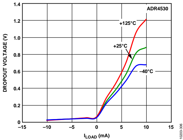
Figure 32. ADR4530 Dropout Voltage vs. Load Current
