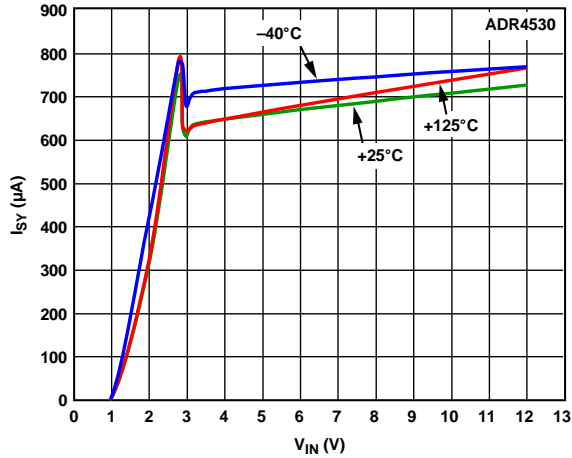
Figure 36. ADR4530 Supply Current vs. Supply Voltage
