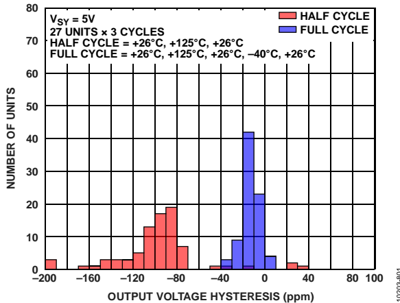
Figure 90. Histogram Showing the Temperature Hysteresis of the Output Voltage (-40°C to +125°C)
