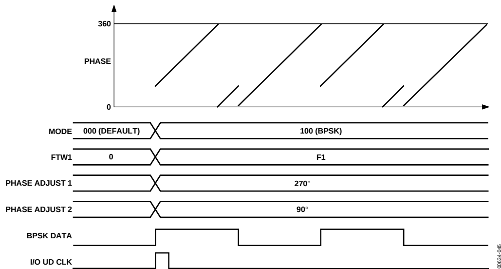
Figure 45. BPSK Mode
