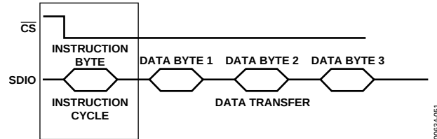
Figure 51. Using SDO as a Read/Write Transfer
