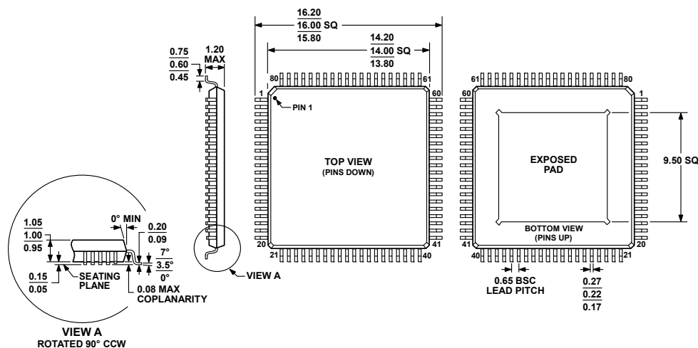
Figure 61. 80-Lead Thin Quad Flat Package, Exposed Pad [TQFP_EP] (SV-80-4) Dimensions shown in millimeters
