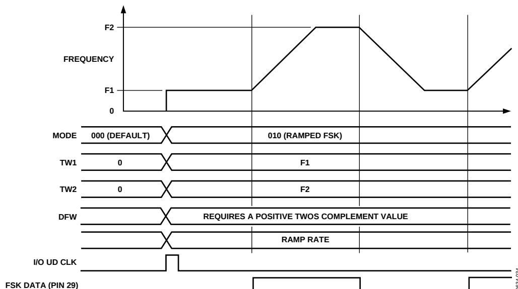
Figure 34. Ramped FSK Mode (Start at F1)
