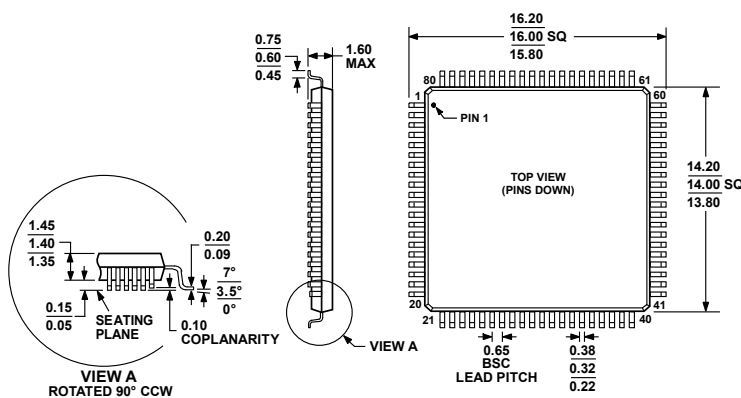
Figure 61. 80-Lead Thin Quad Flat Package, Exposed Pad [TQFP_EP] (SV-80-4) Dimensions shown in millimeters
