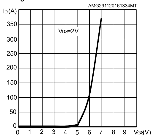
Figure 6: Transfer characteristics
