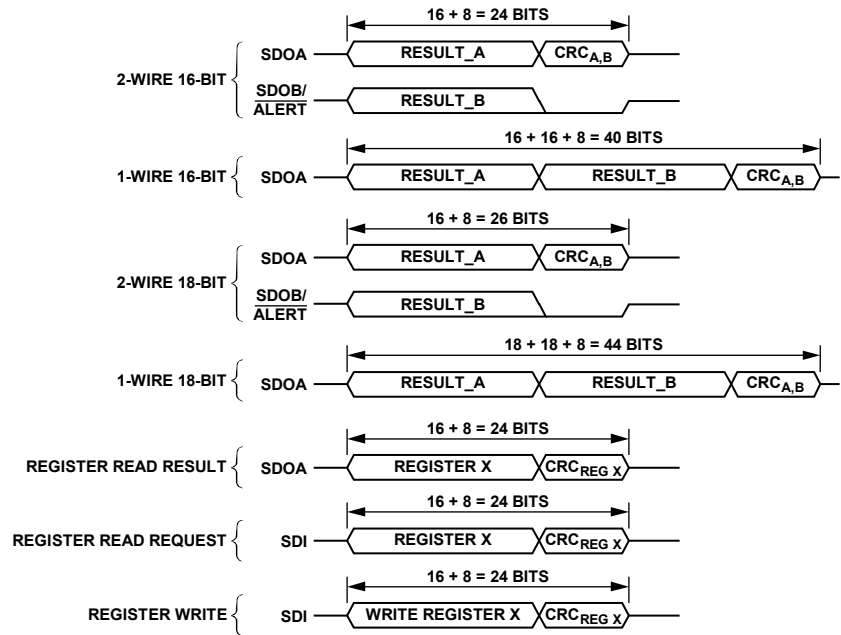
Figure 43. CRC Operation
