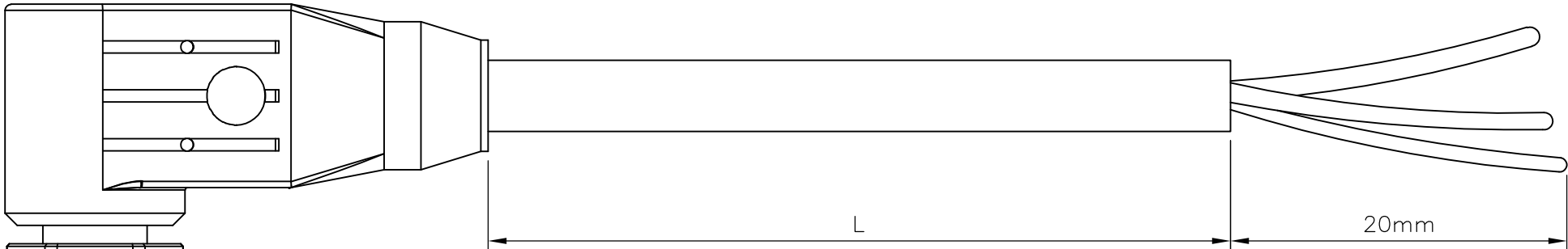
VIEW 'A'
