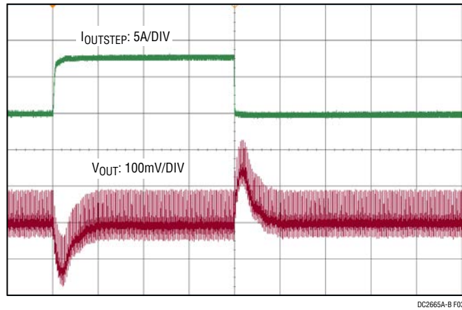
Figure 3. Load Transient (7.5A to 15A) Response Waveform at 12V IN and 1.5V OUT , 50μs/DIV
