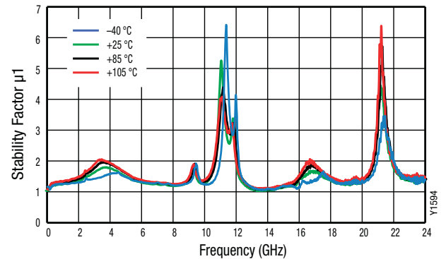
Figure 12. Stability Factor ( \mu_1 ) vs Frequency over Temperature
