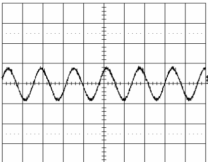
Output voltage ripple (20mV/div.) at: T_{ref} = +25^{\circ}\text{C} , I_O = 6\text{ A} resistive load, V_I = 12.0\text{ V} . Time scale: 2 \mu\text{s} /div. See the filter in the Output ripple and noise section (EMC Specification).
