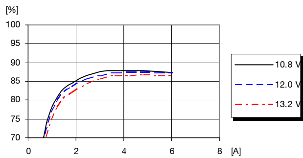
Efficiency
