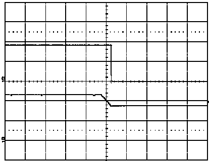
Shut-down enabled by disconnecting V_I at: T_{ref} = +25^{\circ}\text{C} , I_O = 6\text{ A} resistive load, V_I = 12.0\text{ V} . Top trace: output voltage (1.0 V/div.). Bottom trace: input voltage (5 V/div.). Time scale: 5.0 ms/div.
