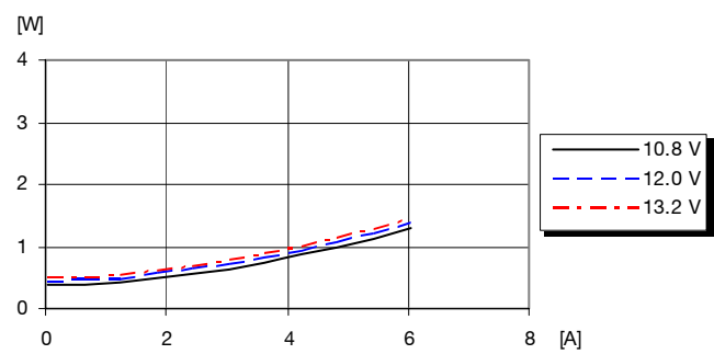
Power Dissipation
