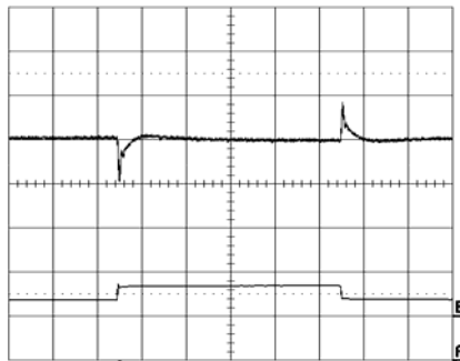
Output voltage response to load current step- change (3-6-3 A) at: T_{ref} = +25^{\circ}\text{C} , V_I = 12.0\text{ V} . Top trace: output voltage (100mV/div.). Bottom trace: load current (10 A/div.). Time scale: 0.1 ms/div.
