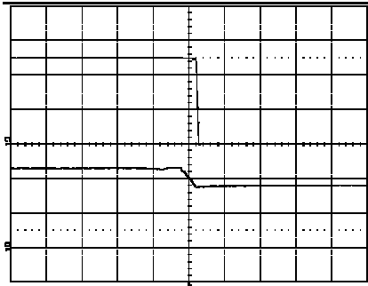
Shut-down enabled by disconnecting V_I at: T_{ref} = +25^{\circ}\text{C} , I_O = 6\text{ A} resistive load, V_I = 12.0\text{ V} . Top trace: output voltage (2.0 V/div.). Bottom trace: input voltage (5 V/div.). Time scale: 2.0 ms/div.
