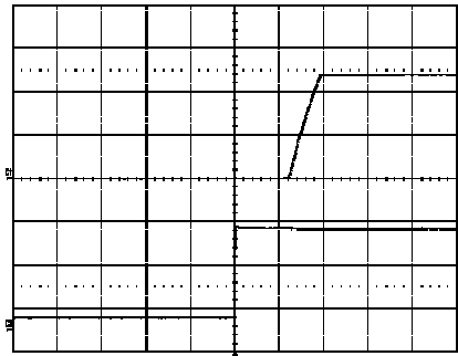
Start-up enabled by connecting V_I at: T_{ref} = +25^{\circ}\text{C} , I_O = 6\text{ A} resistive load, V_I = 12.0\text{ V} . Top trace: output voltage (2.0 V/div.). Bottom trace: input voltage (5 V/div.). Time scale: 10 ms/div.
