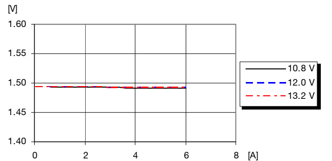
Output Characteristics
