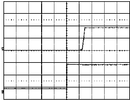
Start-up enabled by connecting V_I at: T_{ref} = +25^{\circ}\text{C} , I_O = 6\text{ A} resistive load, V_I = 12.0\text{ V} . Top trace: output voltage (1.0 V/div.). Bottom trace: input voltage (5 V/div.). Time scale: 10 ms/div.
