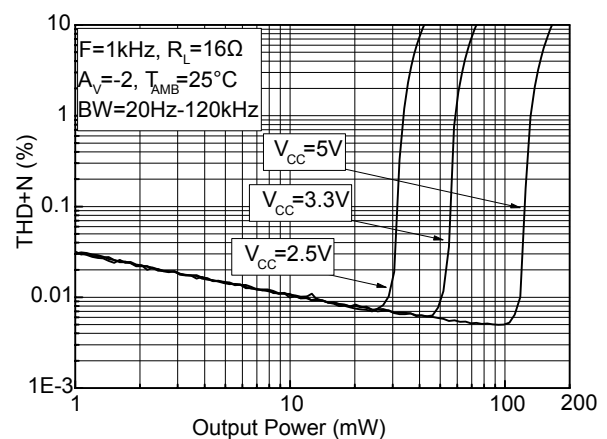
Figure 31. Total harmonic distortion plus noise vs. output power R_L=16\ \Omega , F=1\ \text{kHz} , A_V=-2
