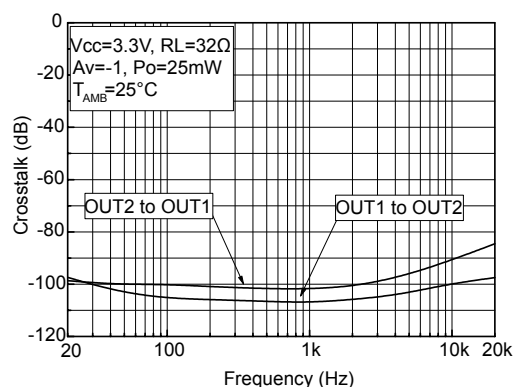
Figure 65. Crosstalk vs. frequency R_L=32\Omega , V_{CC}=3.3V , P_o=25mW
