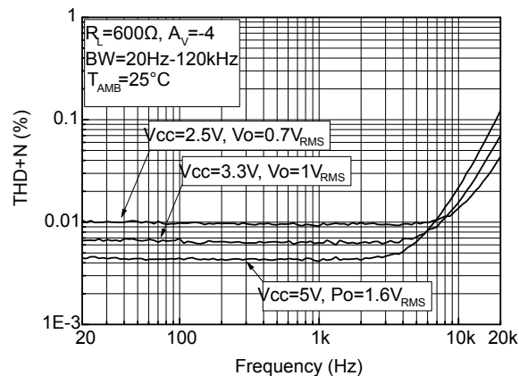
Figure 51. Total harmonic distortion plus noise vs. frequency R_L=600\ \Omega , A_V=-4
