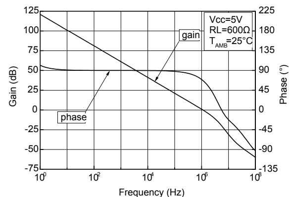
Figure 11. Open-loop frequency response V_{CC} = 5\text{ V} R_L = 600\ \Omega
