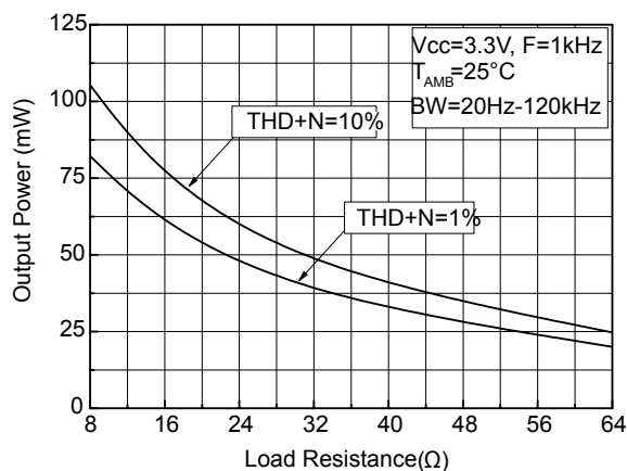
Figure 53. Output power vs. load resistance V_{CC}=3.3\ \text{V}
