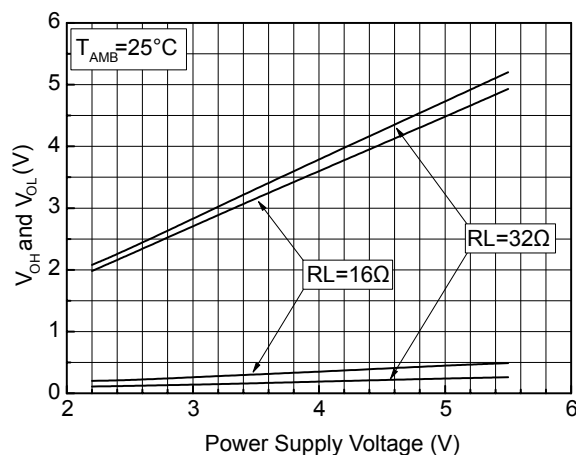
Figure 57. Output power swing vs. power supply voltage
