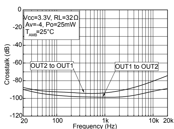
Figure 71. Crosstalk vs. frequency RL=32\ \Omega , V_{CC}=3.3\ V , P_O=25\ mW , A_V=-4
