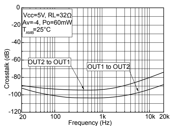
Figure 73. Crosstalk vs. frequency RL=32\ \Omega , V_{CC}=5\ V , P_O=60\ mW
