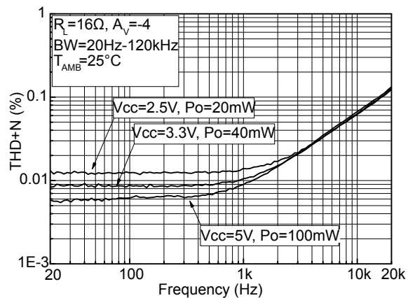
Figure 49. Total harmonic distortion plus noise vs. frequency R_L=16\ \Omega , A_V=-4
