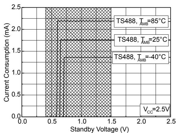
Figure 59. Current consumption vs. standby voltage
