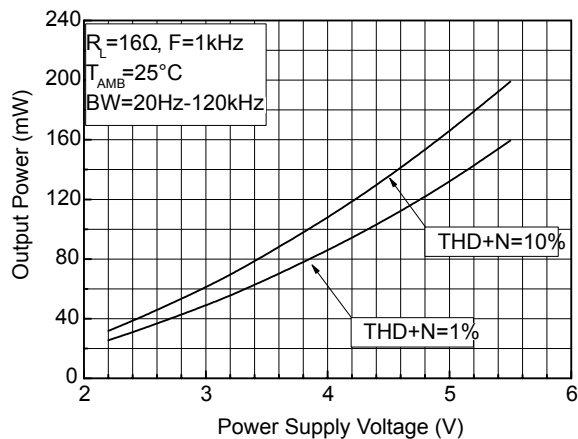
Figure 55. Output power vs. power supply voltage
