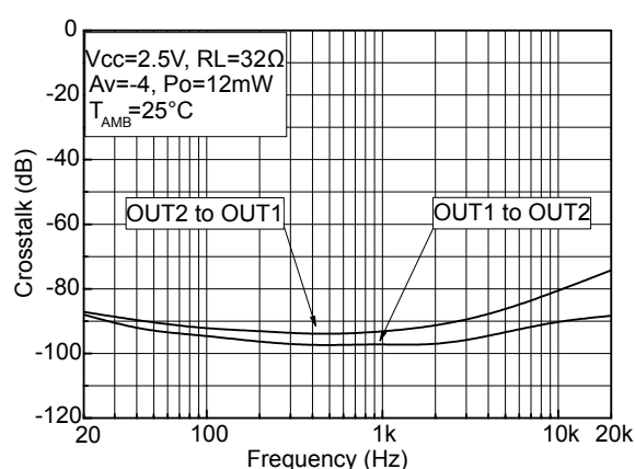
Figure 69. Crosstalk vs. frequency RL=32\ \Omega , V_{CC}=2.5\ V , P_O=12\ mW , A_V=-4
