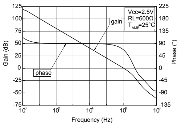
Figure 10. Open-loop frequency response V_{CC} = 2.5\text{ V} R_L = 600\ \Omega
