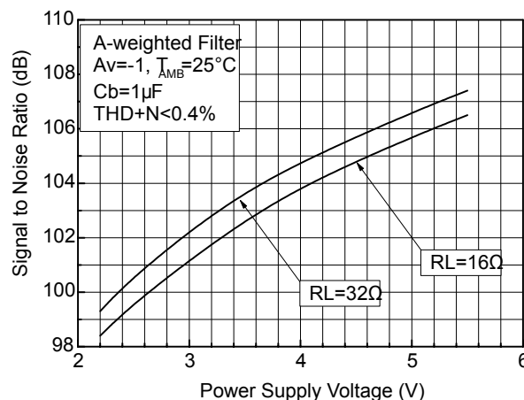
Figure 13. Signal-to-noise ratio vs. power supply voltage A weighted A_V=-1
