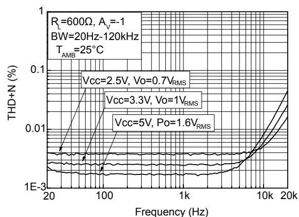
Figure 45. Total harmonic distortion plus noise vs. frequency R_L=600\ \Omega
