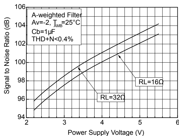
Figure 15. Signal-to-noise ratio vs. power supply voltage A weighted A_V=-2
