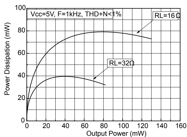
Figure 21. Power dissipation vs. output power per channel V_{CC}=5\text{ V}
