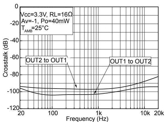
Figure 64. Crosstalk vs. frequency R_L=16\Omega , V_{CC}=3.3V
