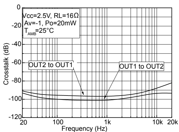
Figure 62. Crosstalk vs. frequency
