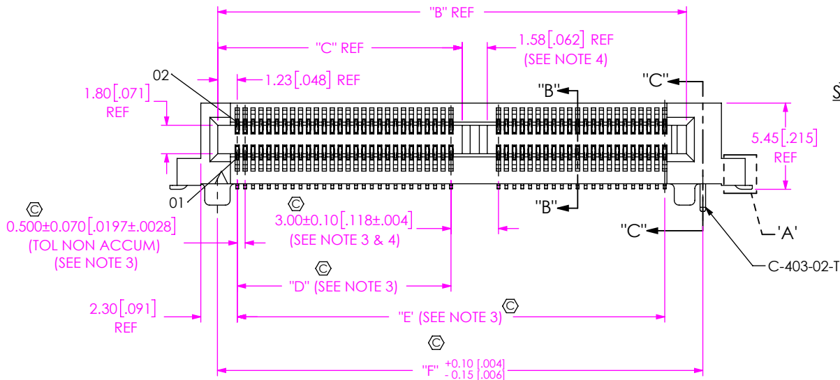
FIG 1 MEC5-050-01-X-D-RA-W2-TR SHOWN
