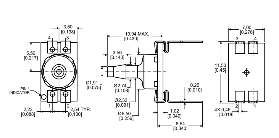
Figure 2. DIP Package Dimensional Drawings (For reference only: mm [in].)
