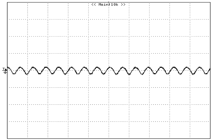
Figure 8: Output ripple & noise at 5Vin, 2.5V/3A out, 50mV/div
