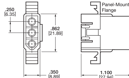
Plug
