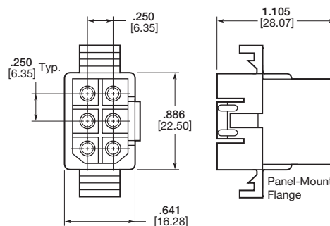
Plug
