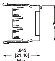
Cap Rear
