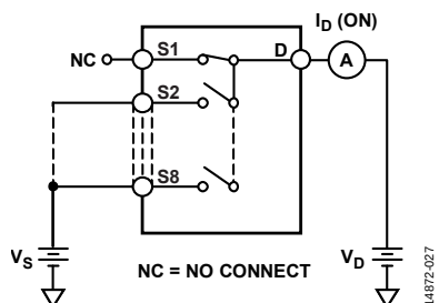
Figure 30. On Leakage
