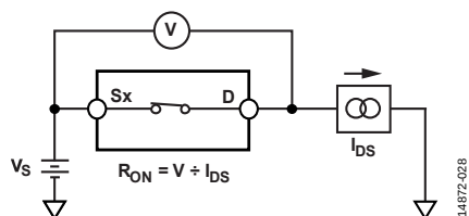
Figure 31. On Resistance
