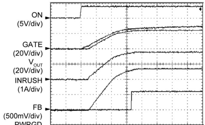
Turn-On Response
