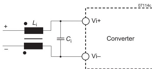
Fig. 15 External filter circuitry
