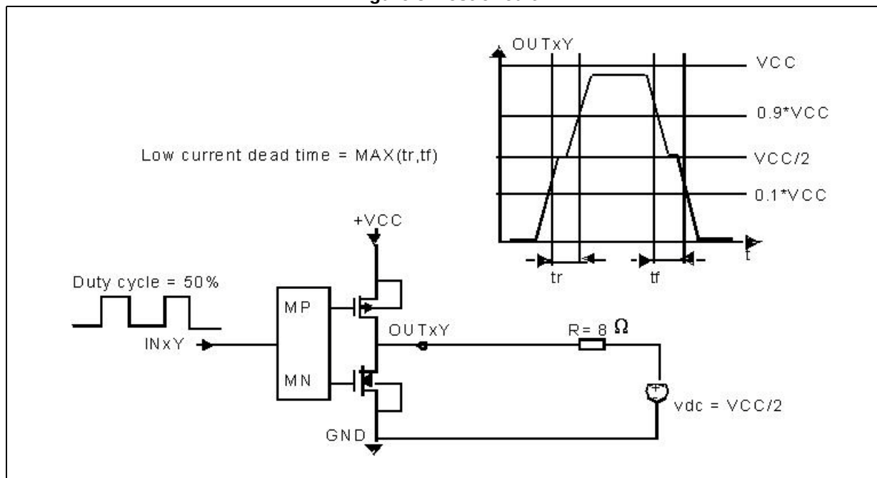
Figure 3. Test circuit
