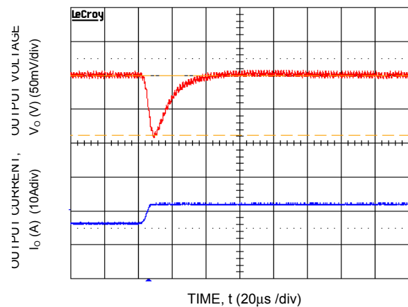
Figure 34. Transient Response to Dynamic Load Change from 50% to 100% at 12V in , C_{out}=5\mu F , C_{Tune}=1500pF & R_{Tune}=330\Omega
