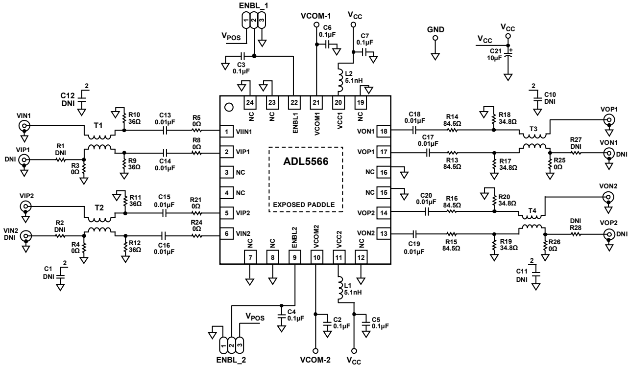
Figure 53. Evaluation Board Schematic
