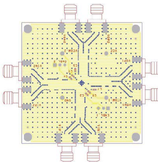
Figure 55. Layout of Evaluation Board, Circuit Side
