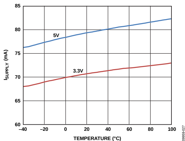
Figure 34. I_{SUPPLY} vs. Temperature, R_L = 200\ \Omega , V_{POS} = 3.3\text{ V} and V_{POS} = 5\text{ V}
