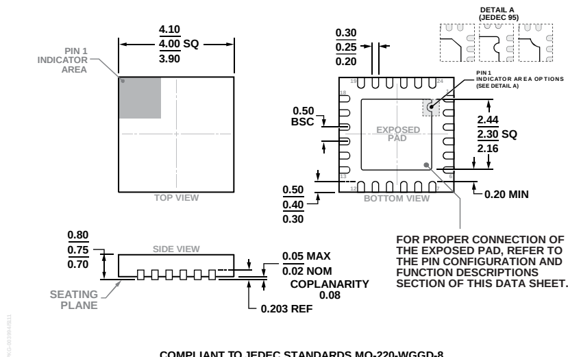
Figure 56. 24-Lead Lead Frame Chip Scale Package [LFCSP] 4 mm × 4 mm Body and 0.75 mm Package Height (CP-24-14)
