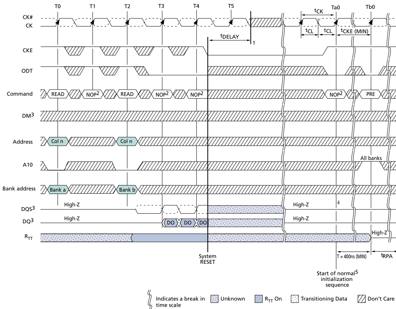
Figure 75: RESET Function
