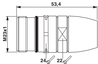
Dimensional drawing
