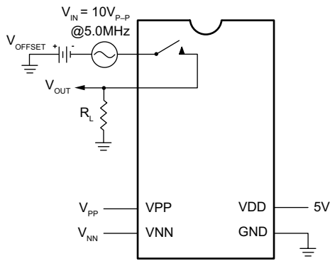
OFF Isolation
