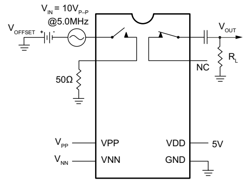
Crosstalk
