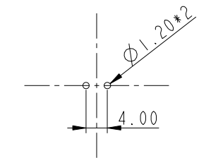
2Pin Male Connector Male Pin PCB Layout
