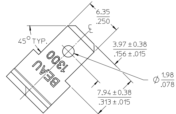
VIEW Z-Z
