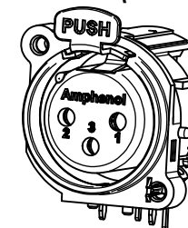
3D VIEW (1:1)
