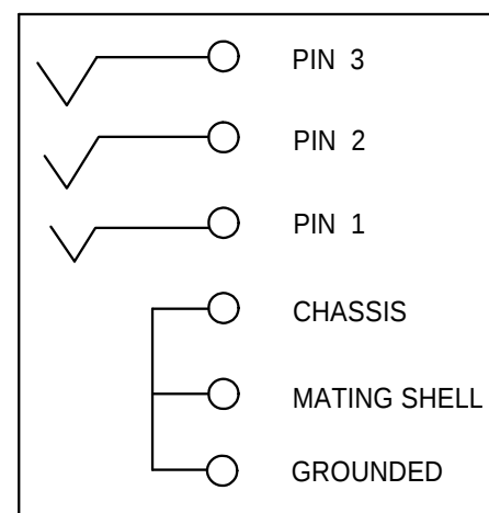
SCHEMATIC CHART
