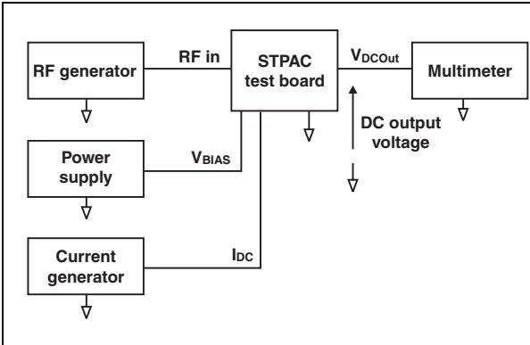
Figure 3. V_{DCout} measurement circuit
