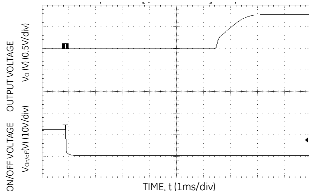
Figure 17 Typical Start-Up Using Remote On/Off with Prebias ( V_{in} = 12.0\text{Vdc} , V_o = 1.8\text{Vdc} , I_o = 1.0\text{A} , V_{bias} = 1.0\text{Vdc} ).
