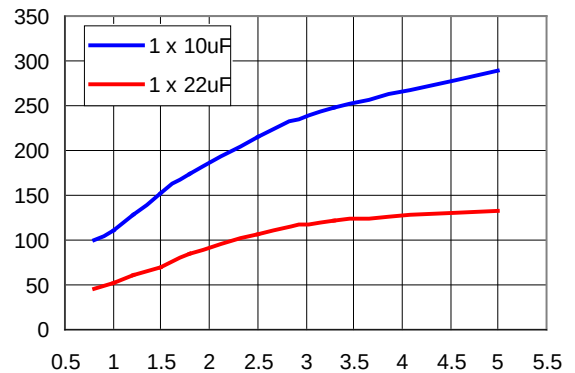
Figure 26. Input ripple voltage for various outputs with 10 μF or a 22 μF ceramic capacitor at the input (full-load).
