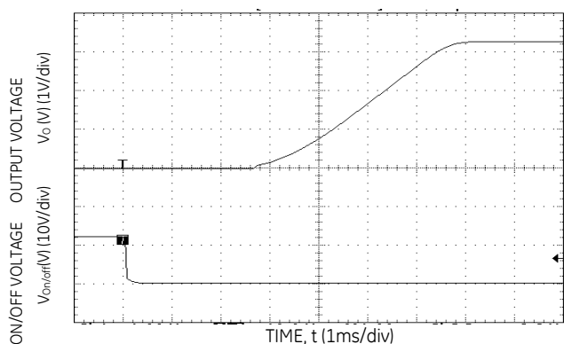
Figure 15. Typical Start-Up Using Remote On/Off with Low-ESR external capacitors (7x150µF Polymer) ( V_{in} = 12.0\text{Vdc} , V_o = 3.3\text{Vdc} , I_o = 3\text{A} , C_o = 1050\text{ }\mu\text{F} ).
