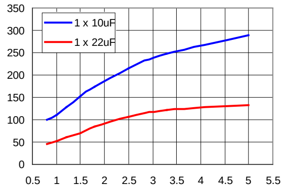
Figure 26. Input ripple voltage for various outputs with 10 µF or a 22 µF ceramic capacitor at the input (full-load).
