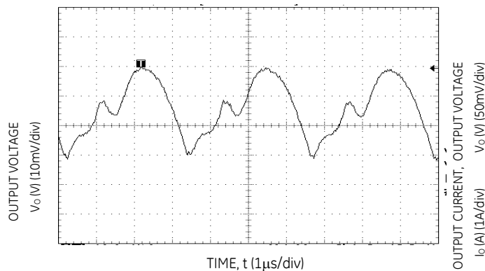
Figure 9. Typical Output Ripple and Noise ( V_{IN} = 12.0Vdc , V_O = 3.3Vdc , I_O=3A ).
