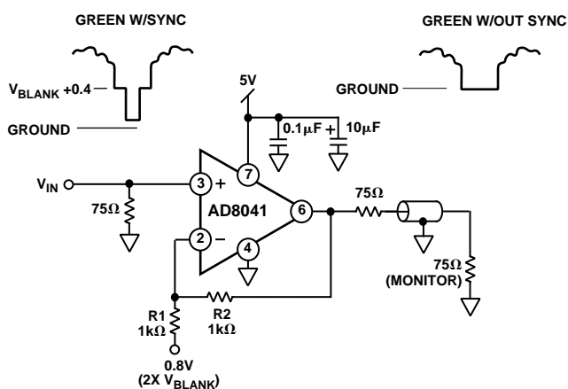
Figure 14. Single-Supply Sync Stripper
