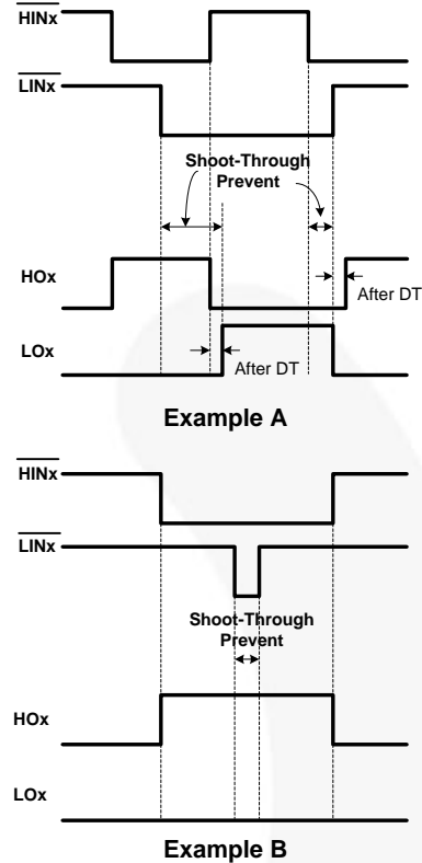
Figure 39. Shoot-Through Protection
