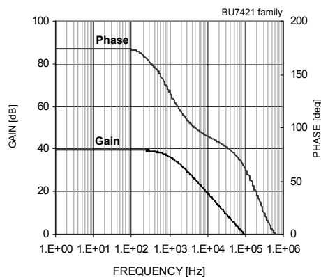
Fig.92 Gain – Frequency
