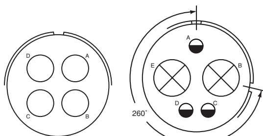
260° Rotation of 32-1
